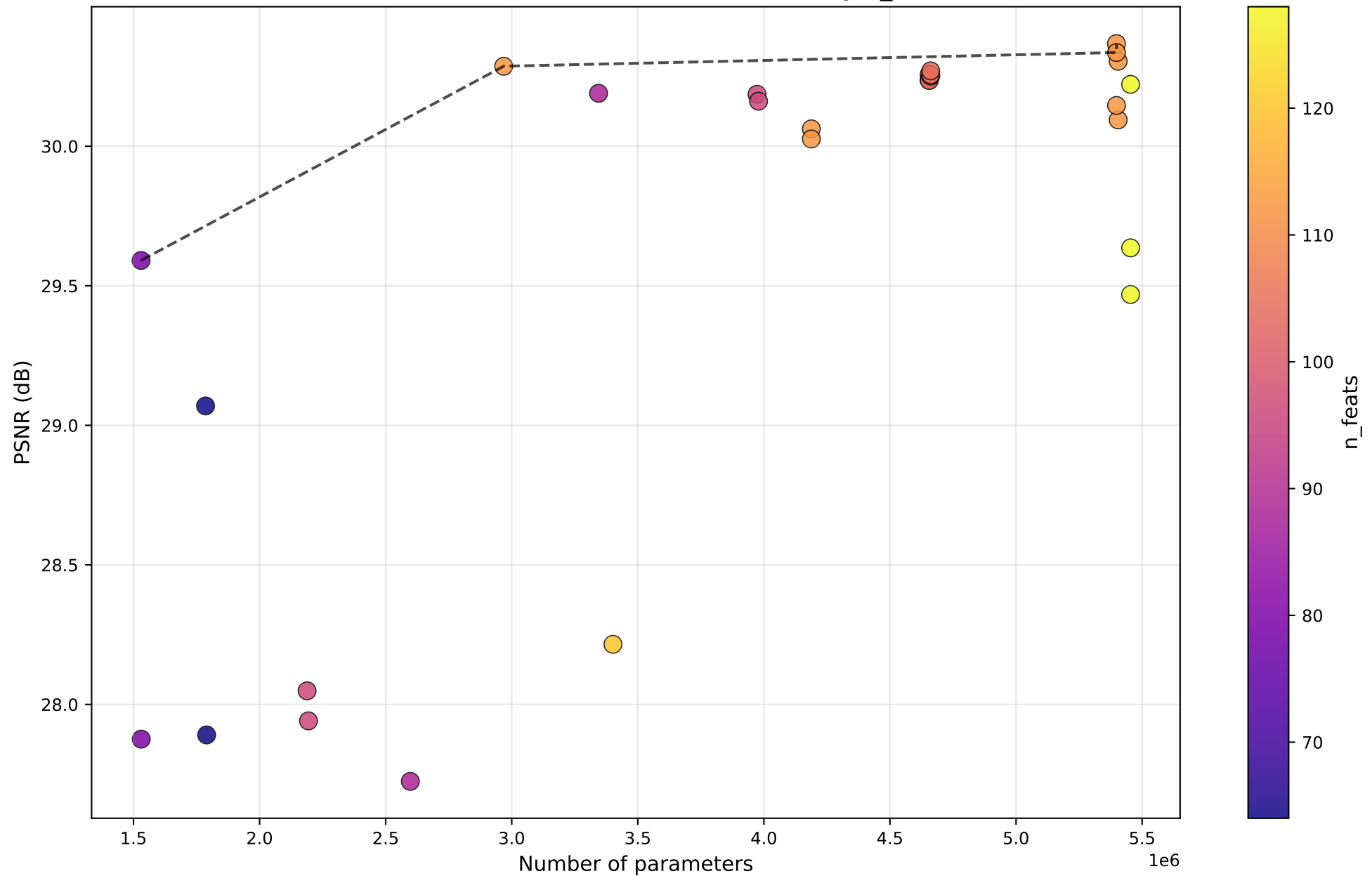
PSNR vs #Params — WaveletAttention — by n_feats
